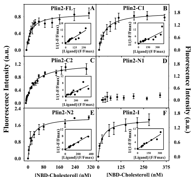
Figure 4. Titration of Plin2 and the deletion mutant proteins with NBD-cholesterol. The binding affinities of Plin2 (A), Plin2-C1 (B), Plin2-C2 (C), Plin2-N1 (D), Plin2-N2 (E), and Plin2-I (F) for NBD-cholesterol were determined using a fluorescence binding assay. The titration of the recombinant proteins with NBD-cholesterol was followed by an increase in fluorescence (excitation 480 nm, emission 540 nm). The data representing the mean \pm SE of three independent measurements were fit to a single binding site model as described in Materials and Methods. Inset, a linear plot of 1/(1 - F/F_{\max}) versus [Ligand]/(F/F_{\max}) was used to determine the K_d as previously described where F represents fluorescence intensity at a given concentration of ligand, F_{\max} is the maximal fluorescence, and [Ligand] is the ligand concentration.
